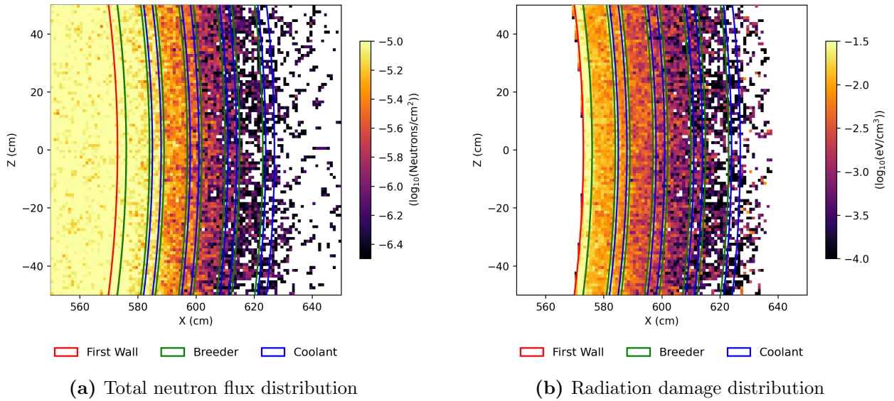
Figure 12: Cross-sectional heatmaps of flux and radiation damage. (a) Illustrates the progressive attenuation of the neutron flux across the material boundaries. (b) Shows the spatial distribution of structural radiation damage.
