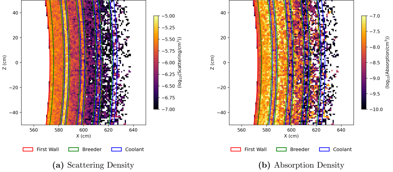
Figure 8: Spatial mapping at \zeta = 0 contrasting thermalising scattering in the water coolant against parasitic absorption in the structural separators.
