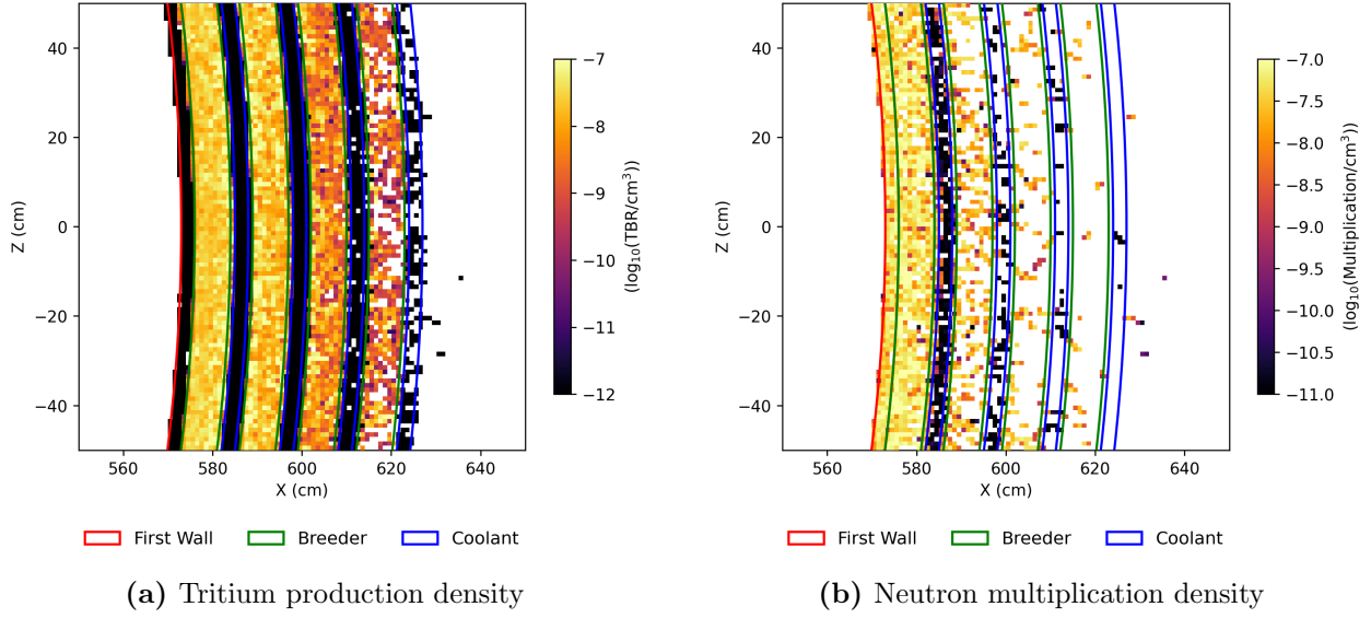
Figure 11: Cross-sectional heatmaps detailing the spatial distribution of key neutronic reactions. (a) Displays the density of tritium breeding reactions, strictly localised within the discrete breeder layers. (b) Illustrates the concentration of neutron multiplication events across the blanket depth. Trace reactions defined in Section 2.1.2 are also highlighted in the non-breeder layers, commonly shaded darker indicating rare events.
