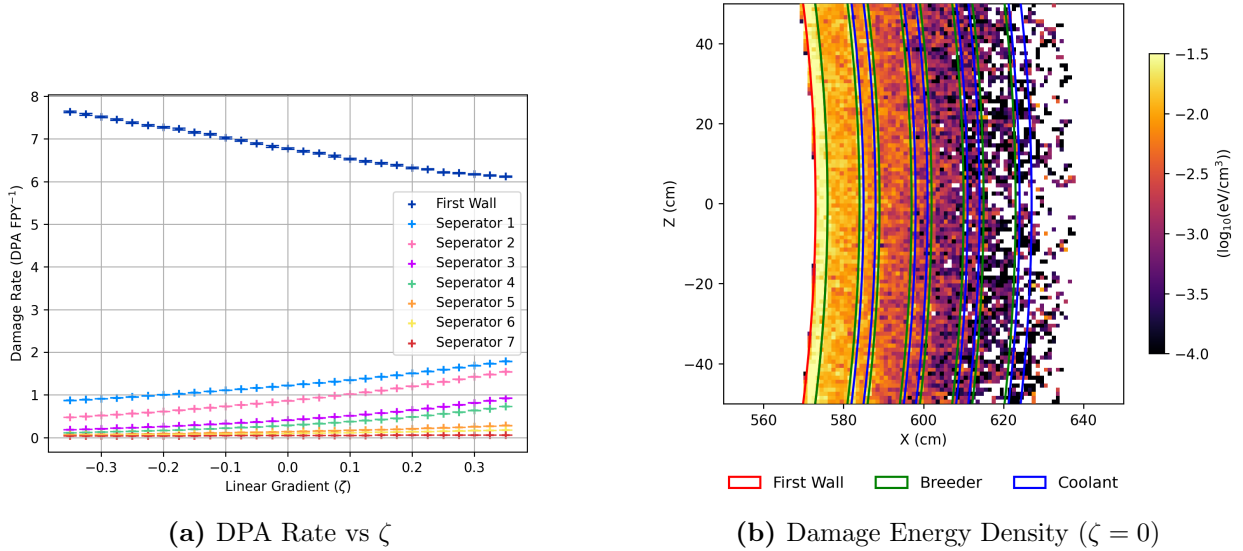
Figure 9: Radiation damage metrics, establishing the strict structural constraints governing first wall and separator lifetimes.
