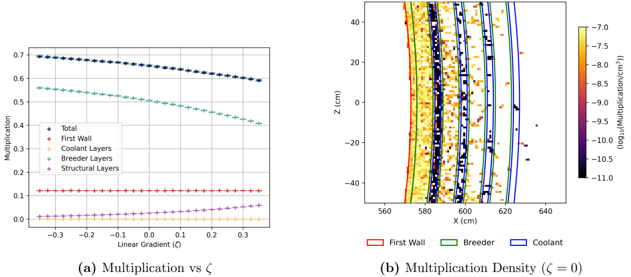
Figure 7: Neutron multiplication rates, highlighting the dependency on high-energy, unmoderated flux in the plasma-facing layers.
