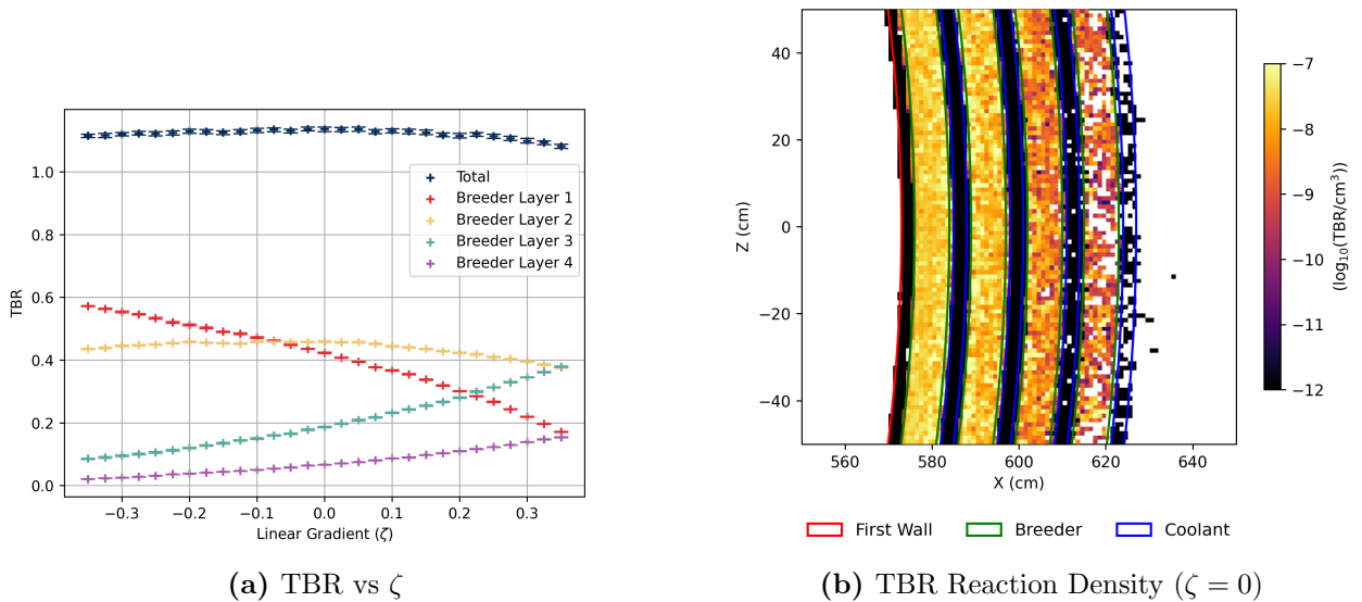
Figure 5: Global and layer-specific TBR performance across the geometric gradient, paired with the spatial distribution of breeding reactions.
